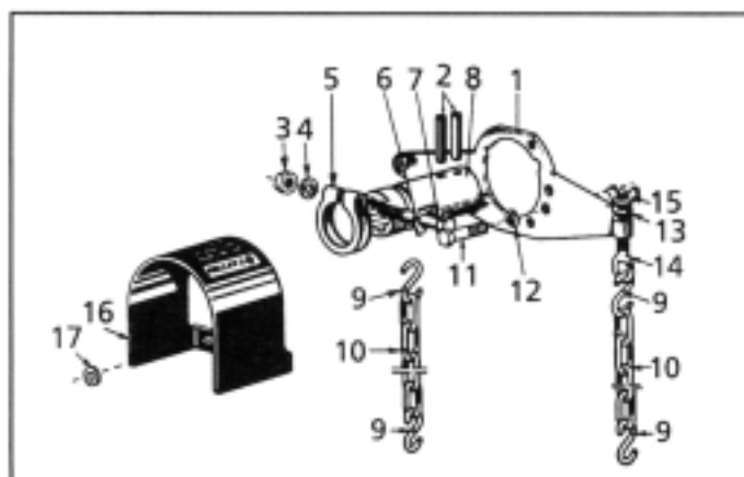
Figure 8. 9910-Kit 1708 1-3/8" Female PTO Adapter, Safety Shield, Torque Arm and Chains
