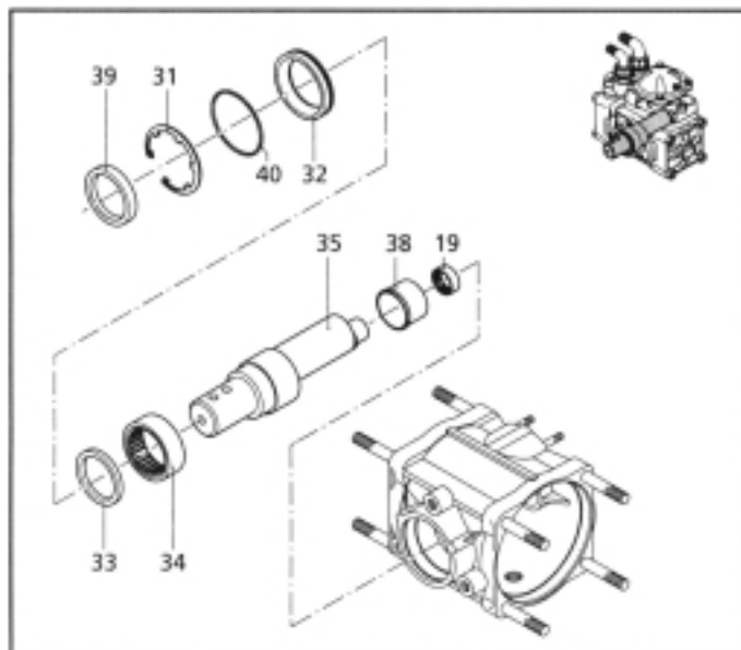
Figure 7. Parts Illustrations for Model 9910-D70
