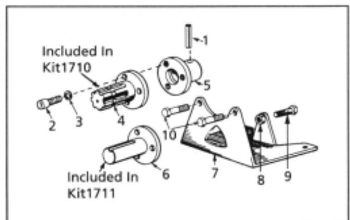
Figure 9. 9910-Kit 1710 1-3/8" Male PTO Shaft and Base Kit 9910-Kit 1711 1" Solid Shaft and Base Kit
